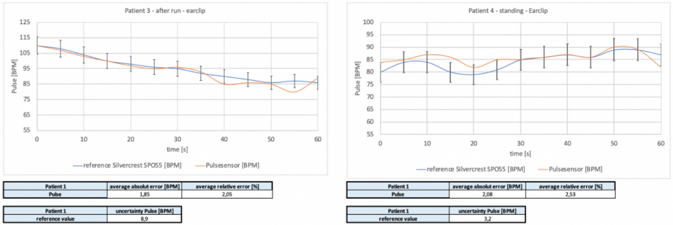
Figure 86: Pulse measurements and comparison to reference device with error and uncertainty calculation for patient 3 and 4
