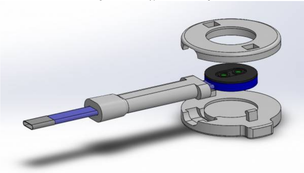
Figure 48: Exploded View Prototype Sensor Casing
