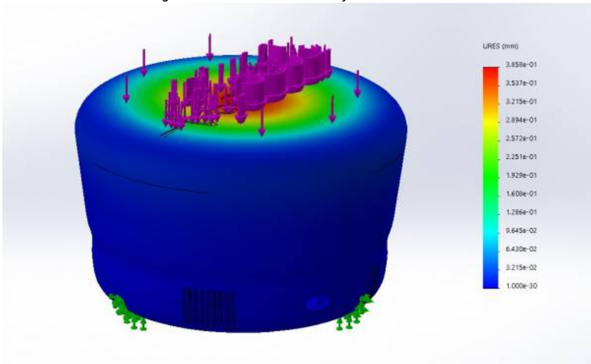
Figure 68: Displacement material by force of 100 N
