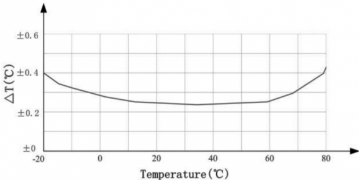
Figure 70: The maximum temperature error [235]
