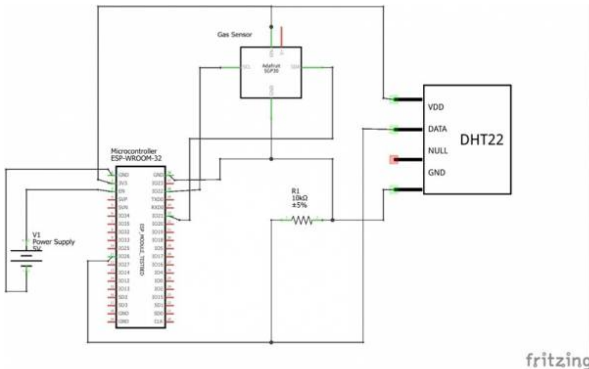
Figure 65: Home Station Schematic Drawing
