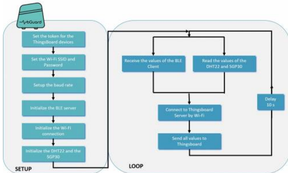
Figure 94: Flowchart for the Server- Arduino code
