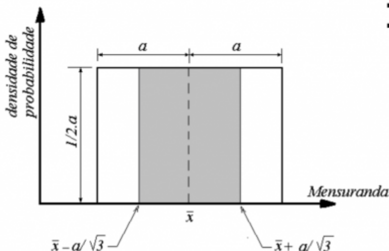
Figure 72: Rectangular approach for measurements
