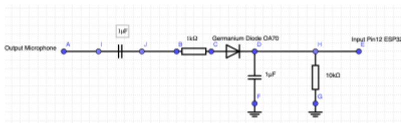
Figure 89: Microphonesignal filter for cry detection
