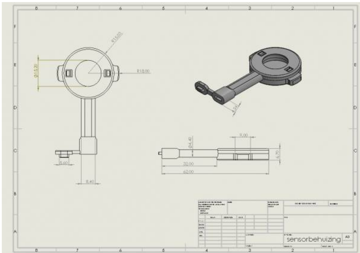
Figure 55: Sensor casing 2D Structural Draft
