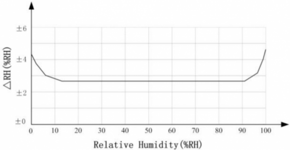
Figure 69: Error of RH at 25 °C [234]
