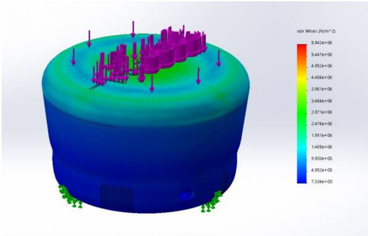
Figure 67: Tension material by force of 100 N
