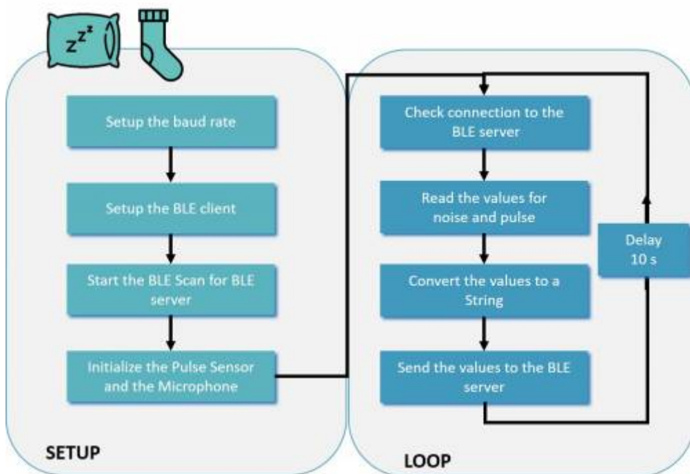
Figure 93: Flowchart for the Client- Arduino code
