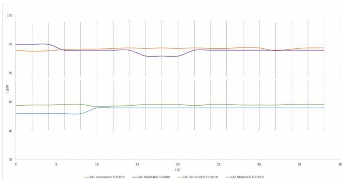
Figure 91: Frequency dependence of noise level for extrema for 500 Hz and 100 Hz with 5 % acceptance range
