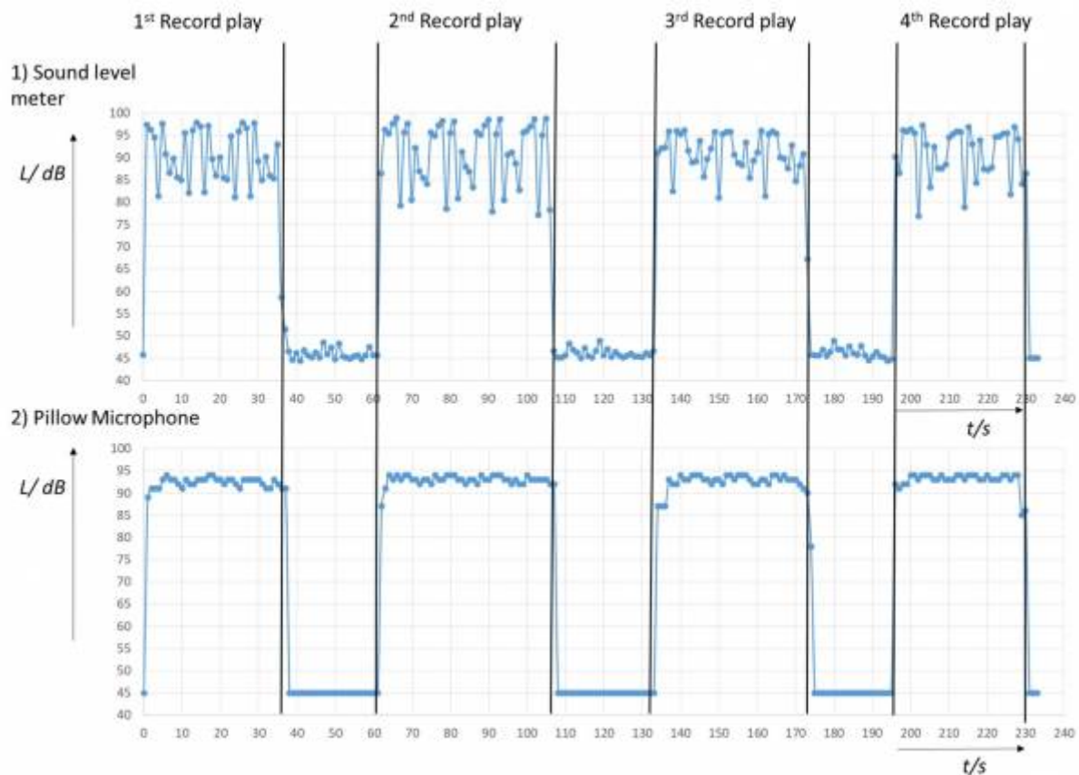
Figure 92: Diagrams of the baby crying record with the sound level L over the time t with 1) Sound level meter and 2) Pillow Microphone
